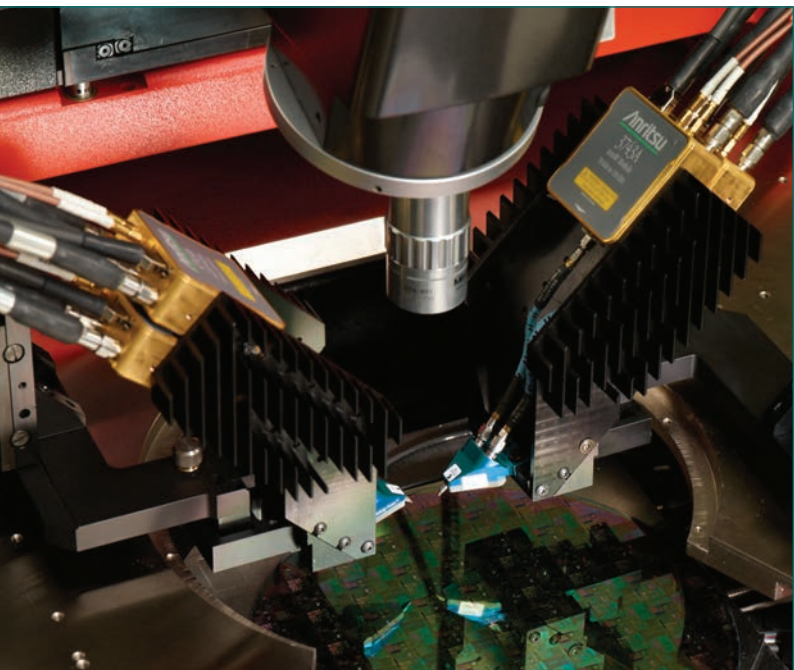
This figure demonstrates the convenience of setting up a 4 port differential broadband measurement to 110 GHz using the compact Anritsu mm-wave modules.
