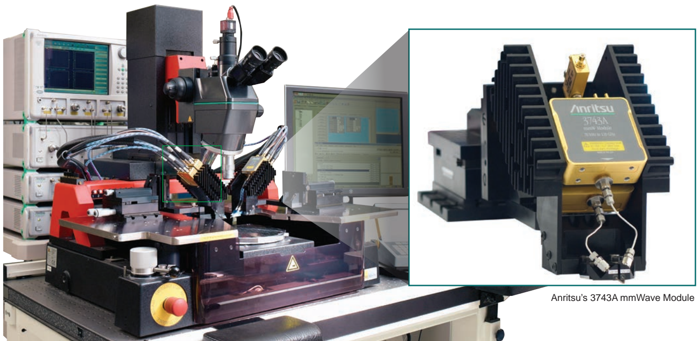
Anritsu's VectorStar ME7838A integrated into an on-wafer probe station.
