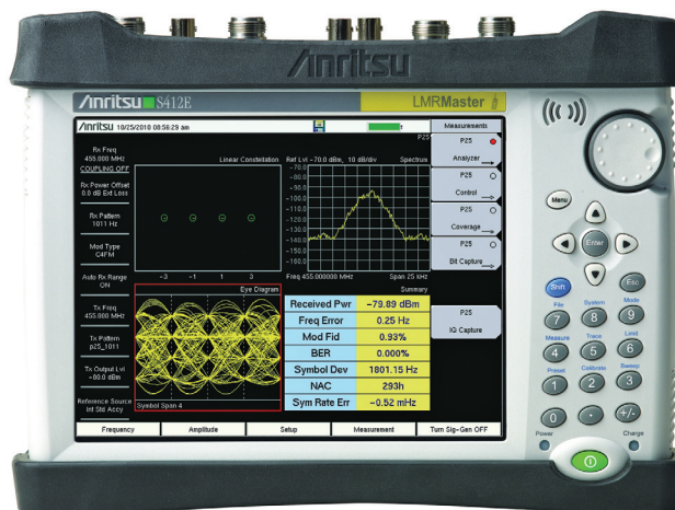
LMR Master™ S412E featuring 8.4 inch Daylight Viewable Touchscreen Compact Size: 273 mm x 199 mm x 91 mm, (10.7 inch x 7.8 inch x 3.6 inch), Lightweight: 3.6 kg, (7.9 lbs)
